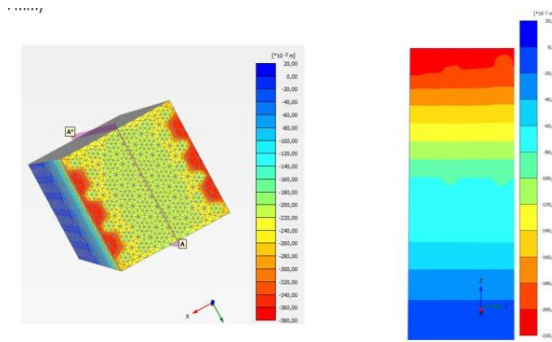
Figure 4. Settlement results for the 3D model (settlement in the cross-section A-A max. 220mm).
